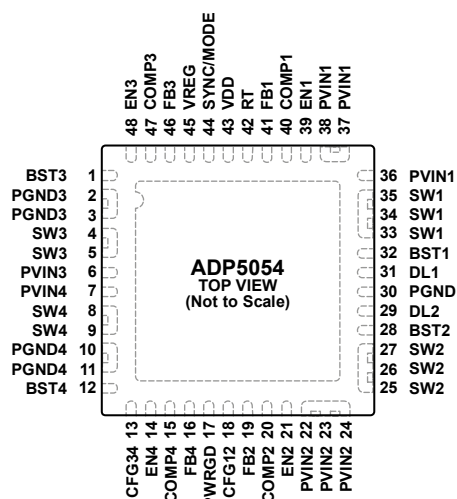
Figure 3. Pin Configuration
