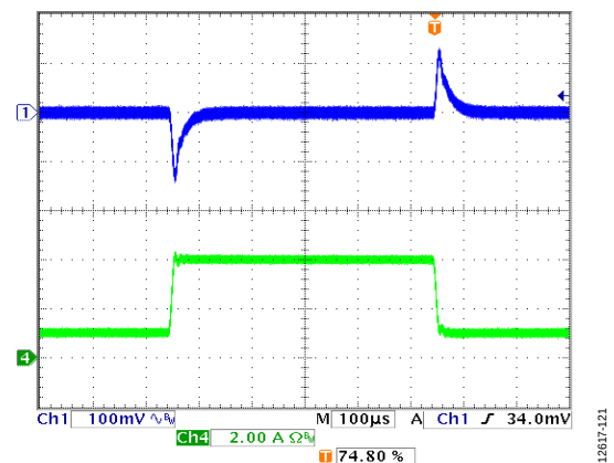
Figure 21. Channel 1/Channel 2 Load Transient, 1A to 4A, V_{IN} = 12V , V_{OUT} = 3.3V , f_{SW} = 600kHz , L = 2.2\mu H , C_{OUT} = 47\mu F \times 2 , Channel 1 = V_{OUTx} , Channel 4 = I_{OUTx}
