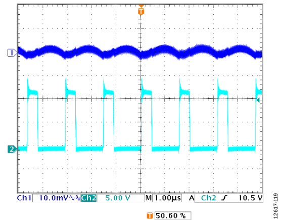
Figure 19. Steady State Waveform at Heavy Load, V_{IN} = 12V , V_{OUT} = 3.3V , Output Load Current ( I_{OUT} ) = 3A, f_{SW} = 600kHz , L = 4.7\mu H , C_{OUT} = 47\mu F \times 2 , FPWM Mode, Channel 1 = V_{OUTx} , Channel 2 = SWx
