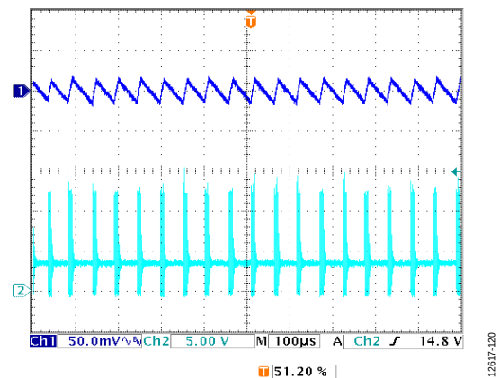
Figure 20. Steady State Waveform at Light Load, V_{IN} = 12V , V_{OUT} = 3.3V , I_{OUT} = 30mA , f_{SW} = 600kHz , L = 4.7\mu H , C_{OUT} = 47\mu F \times 2 , Automatic PWM/PSM Mode, Channel 1 = V_{OUTx} , Channel 2 = SWx
