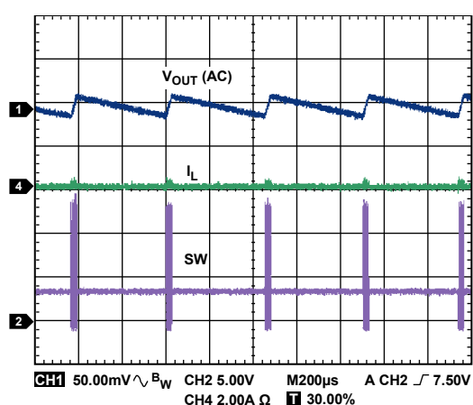
Figure 27. Power Saving Mode, V_{OUT} = 3.3\text{ V} , V_{IN} = 12\text{ V}
