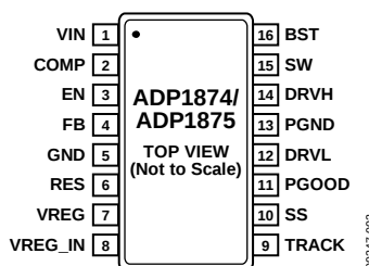
Figure 3. Pin Configuration
