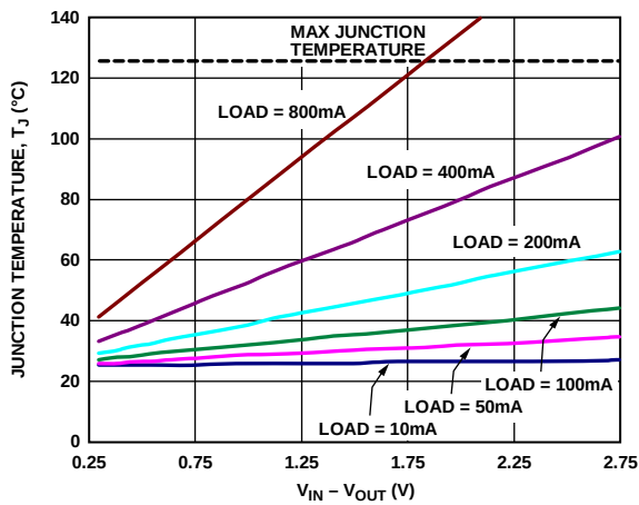
Figure 37. 500 mm 2 of PCB Copper, T_A = 25^\circ\text{C} , LFCSP
