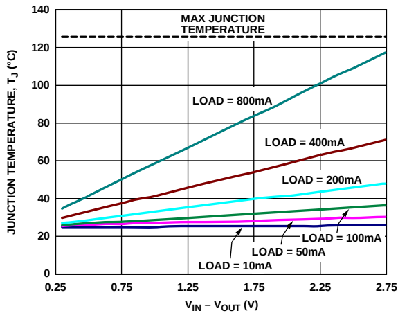
Figure 36. 6400 mm 2 of PCB Copper, T_A = 25^\circ\text{C} , LFCSP
