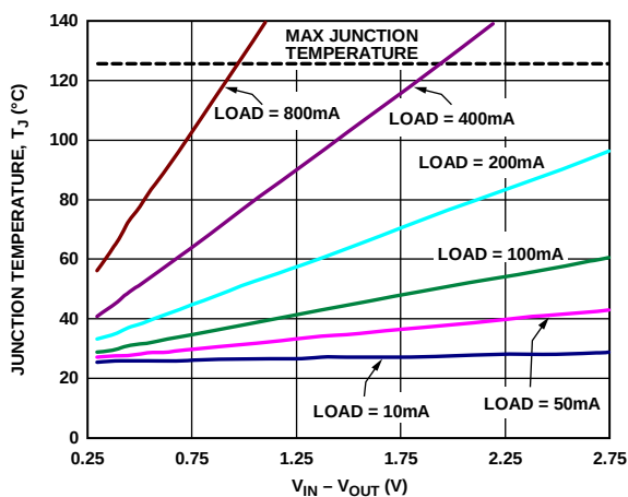
Figure 38. 0 mm 2 of PCB Copper, T_A = 25^\circ\text{C} , LFCSP
