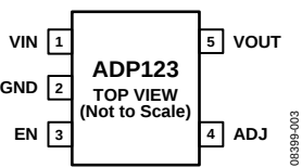
Figure 7. ADP123 TSOT Adjustable Output Pin Configuration
