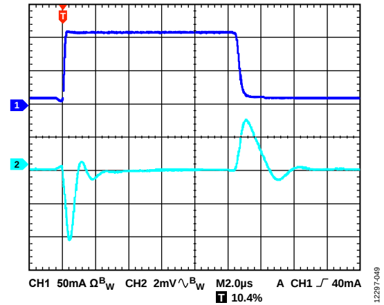
Figure 49. Load Transient Response, I_{LOAD} = 10mA to 110mA , V_{OUT} = 5V , V_{IN} = 5.5V , CH1 = I_{LOAD} , CH2 = V_{OUT}
