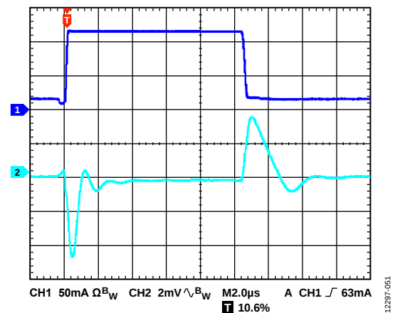
Figure 51. Load Transient Response, I_{LOAD} = 10mA to 110mA , Adjustable Version, V_{OUT} = 1.2V , V_{IN} = 2.5V , CH1 = I_{LOAD} , CH2 = V_{OUT}
