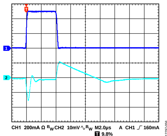
Figure 56. Output Transient Response, V_{OUT} = 5\text{ V} , C_{OUT} = 4.7\text{ }\mu\text{F}
