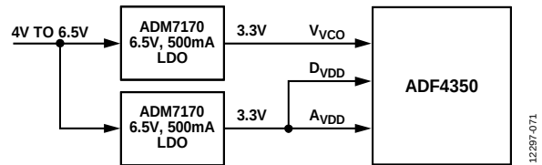
Figure 68. RF PLL/VCO Power
