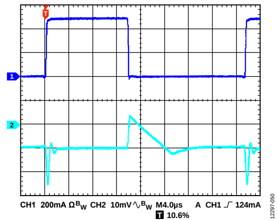
Figure 50. Load Transient Response, I_{LOAD} = 10mA to 510mA , Adjustable Version, V_{OUT} = 1.2V , V_{IN} = 2.5V , CH1 = I_{LOAD} , CH2 = V_{OUT}
