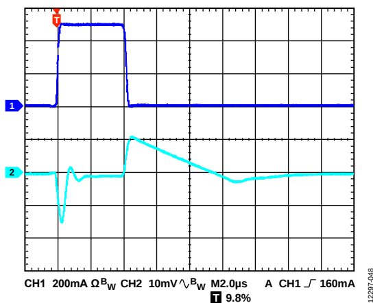
Figure 48. Load Transient Response, I_{LOAD} = 10mA to 510mA , V_{OUT} = 5V , V_{IN} = 5.5V , CH1 = I_{LOAD} , CH2 = V_{OUT}
