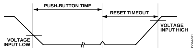
Figure 12. Push-Button Reset Timing Diagram
