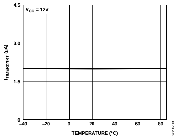
Figure 18. Timer Pull-Down Current, Retry ( I_{\text{TIMERDNRRT}} ) vs. Temperature
