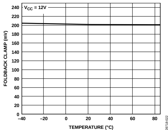
Figure 22. Foldback Clamp vs. Temperature
