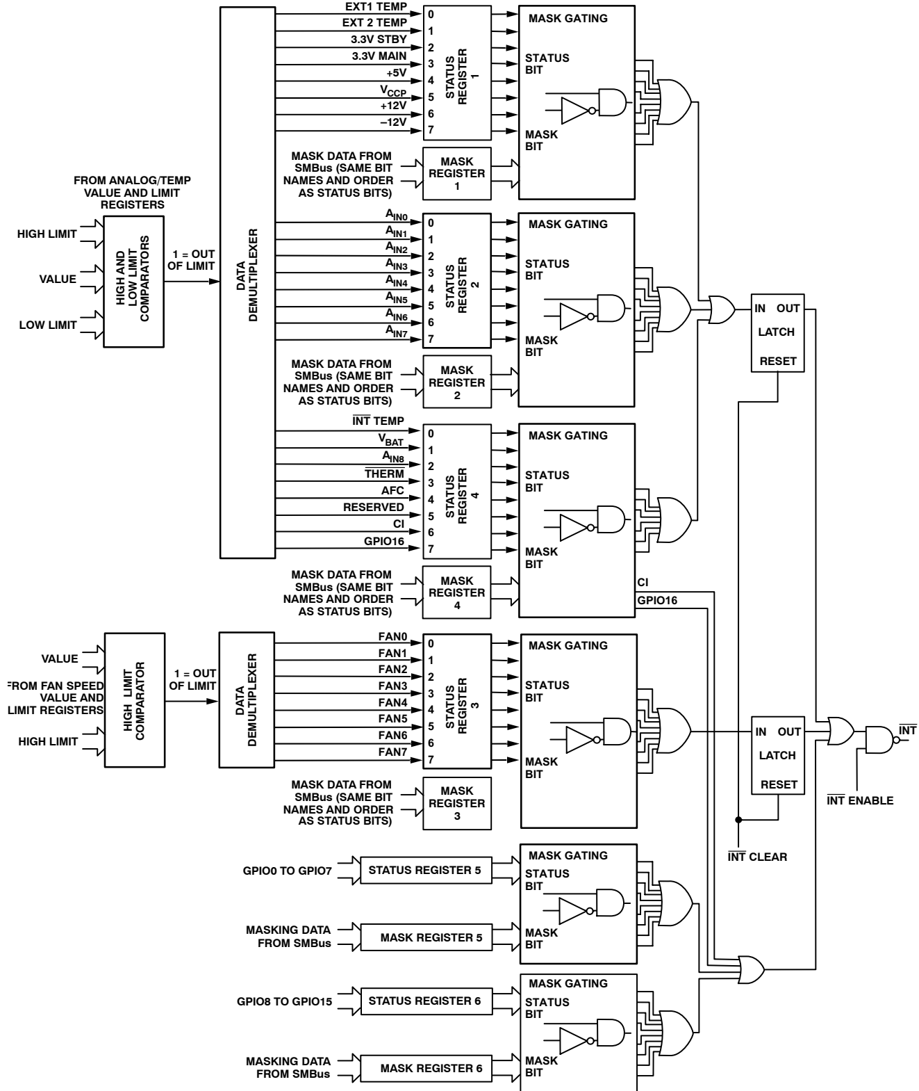
Figure 52. Interrupt Structure
