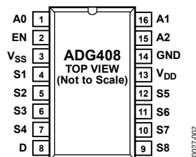
Figure 2. ADG408 Pin Configuration
