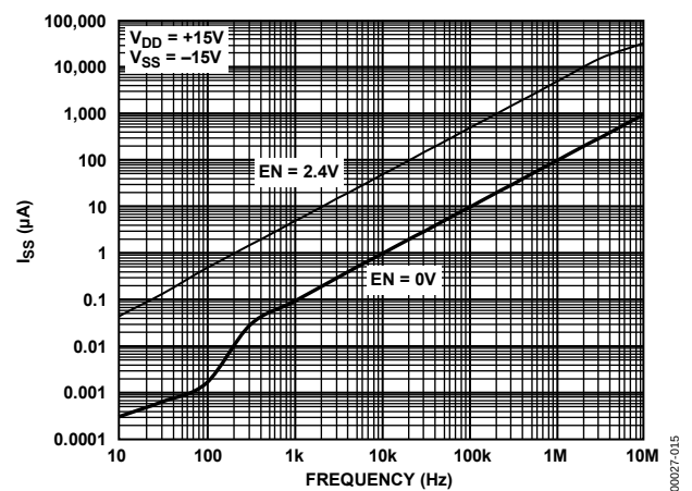
Figure 15. Negative Supply Current vs. Switching Frequency
