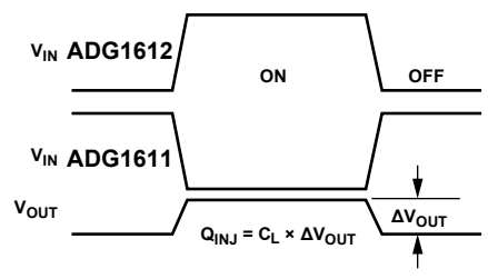
Figure 33. Charge Injection
