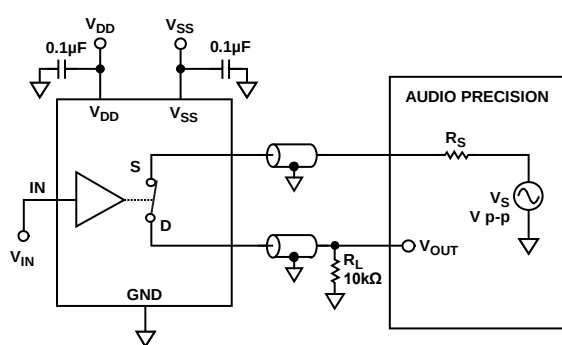
Figure 31. THD + Noise
