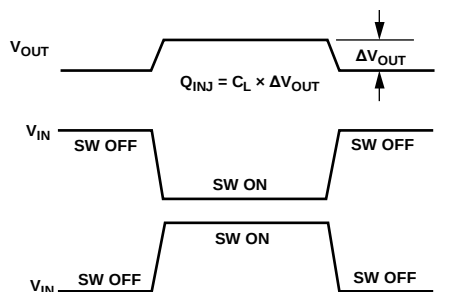
Figure 27. Charge Injection
