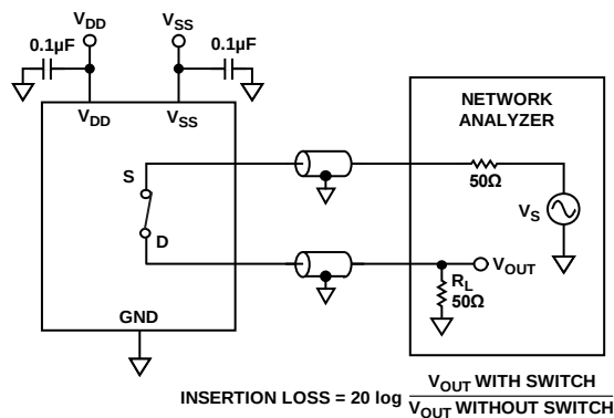
Figure 29. Bandwidth
