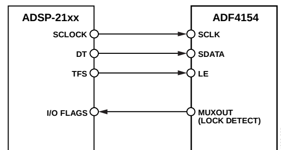
Figure 22. ADSP-21xx-to-ADF4154 Interface
