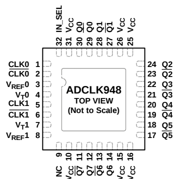
Figure 2. Pin Configuration
