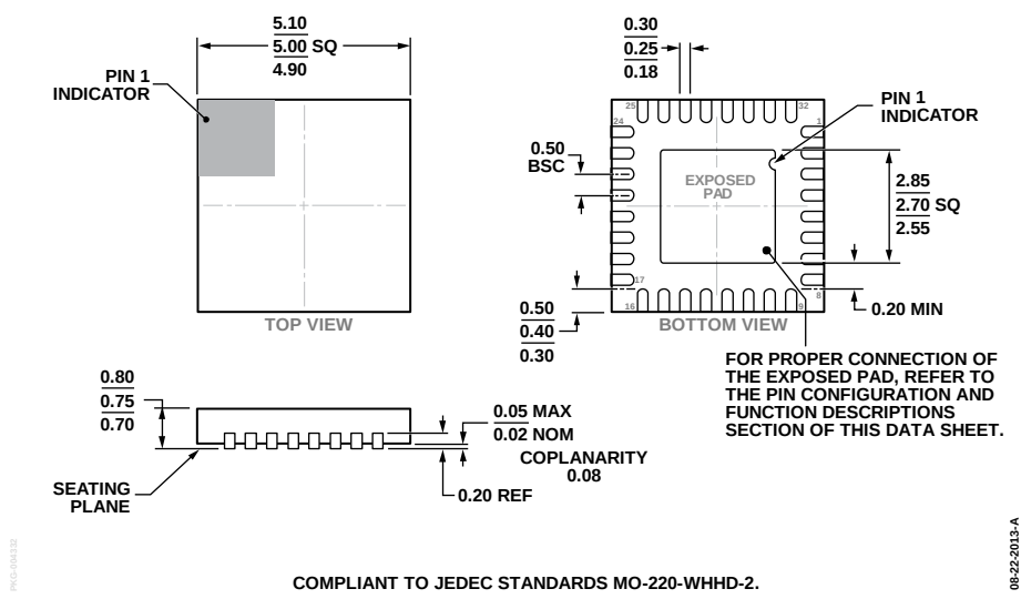
COMPLIANT TO JEDEC STANDARDS MO-220-WHHD-2. Figure 24. 32-Lead Lead Frame Chip Scale Package [LFCSP] 5 mm × 5 mm Body and 0.75 mm Package Height (CP-32-21) Dimensions shown in millimeters
