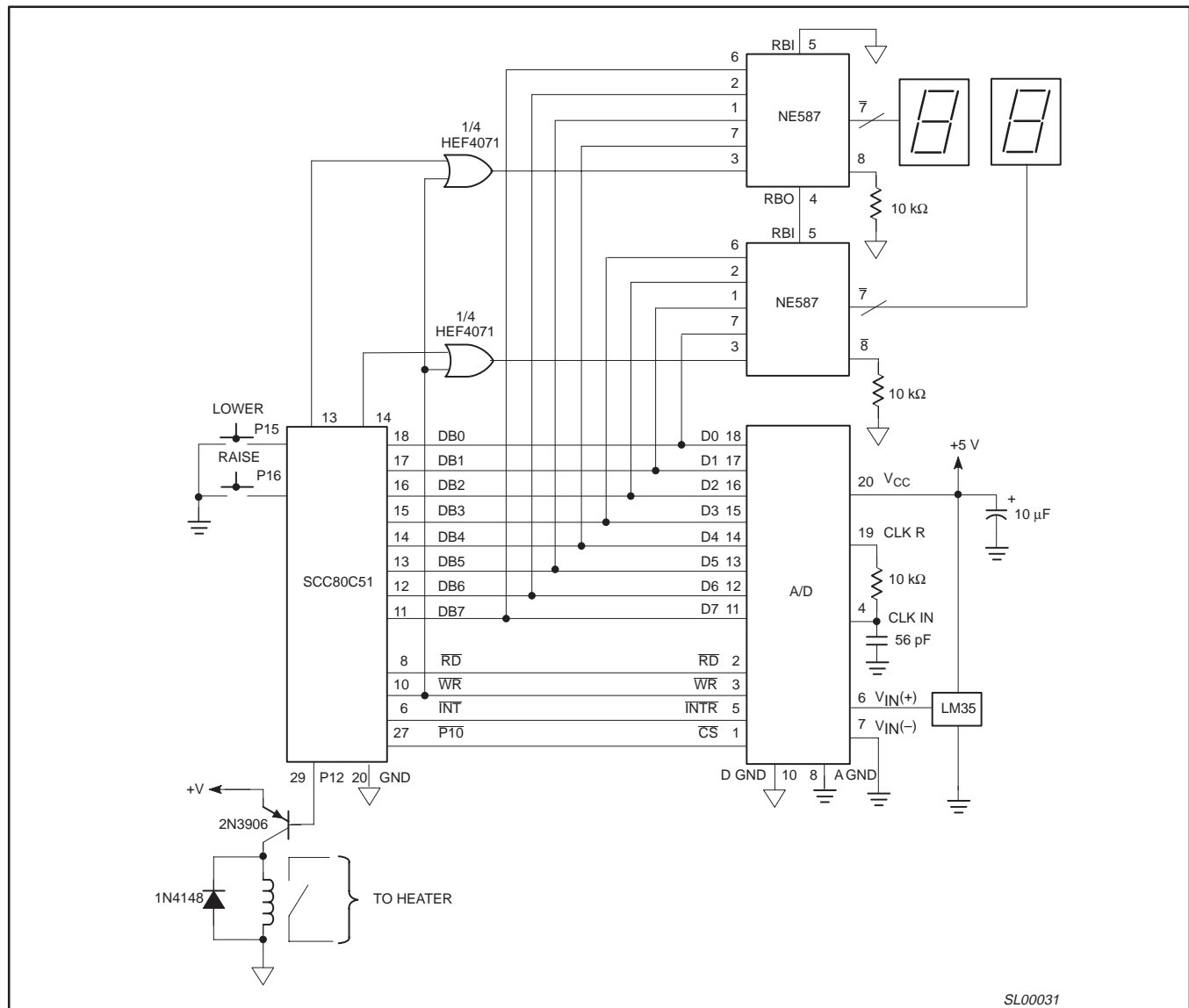
Figure 16. Digital Thermostat
