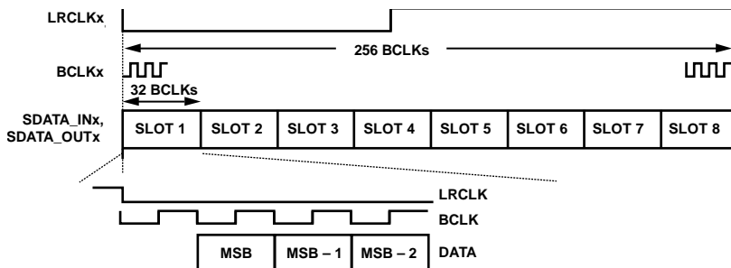
Figure 25. TDM Mode
