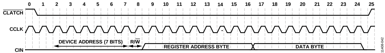
Figure 40. SPI Write to ADAU1979 Clocking (Single-Word Write Mode)
