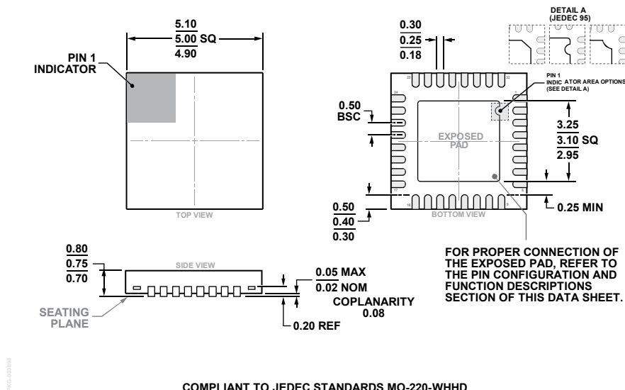
COMPLIANT TO JEDEC STANDARDS MO-220-WHHD Figure 28. 32-Lead Lead Frame Chip Scale Package [LFCSP] 5 mm × 5 mm Body and 0.75 mm Package Height (CP-32-7) Dimensions shown in millimeters
