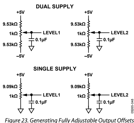
Figure 23. Generating Fully Adjustable Output Offsets
