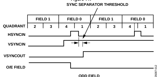
Figure 12. Vsync Filter—Odd/Even
