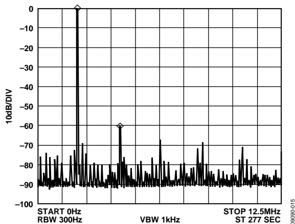
Figure 15. f_{MCLK} = 25 MHz, f_{OUT} = 2.1 MHz, Frequency Word = 0x15810625
