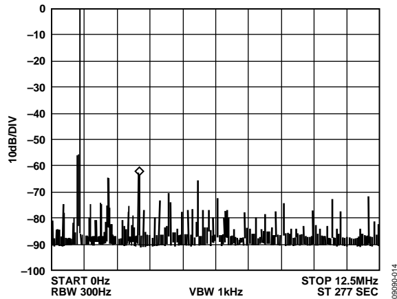
Figure 14. f_{MCLK} = 25 MHz, f_{OUT} = 1.1 MHz, Frequency Word = 0xB439581
