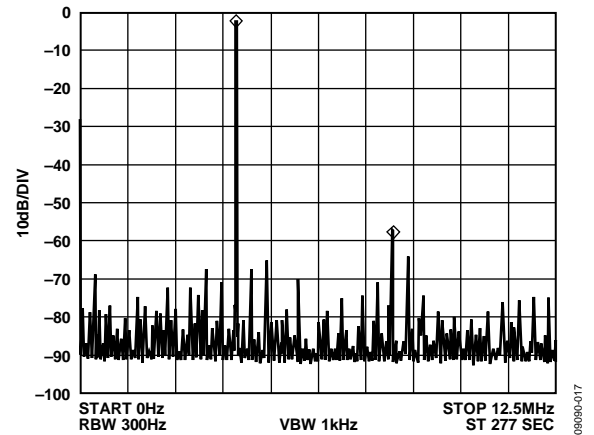
Figure 17. f_{MCLK} = 25 MHz, f_{OUT} = 4.1 MHz, Frequency Word = 0x29FBE76D
