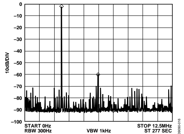
Figure 16. f_{MCLK} = 25 MHz, f_{OUT} = 3.1 MHz, Frequency Word = 0x1FBE76C9
