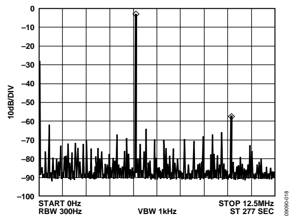
Figure 18. f_{MCLK} = 25 MHz, f_{OUT} = 5.1 MHz, Frequency Word = 0x34395810
