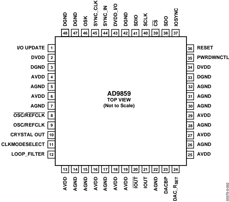
Figure 3. 48-Lead TQFP/EP
