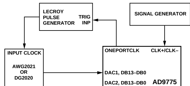
Figure 101. Test Configuration for AD9775 in Two-Port Mode with PLL Enabled, Signal Generator Frequency = Input Data Rate, DAC Output Data Rate = Signal Generator Frequency \times Interpolation Rate
