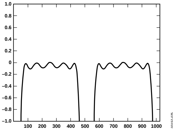
Figure 75. Hilbert Transform Ripple
