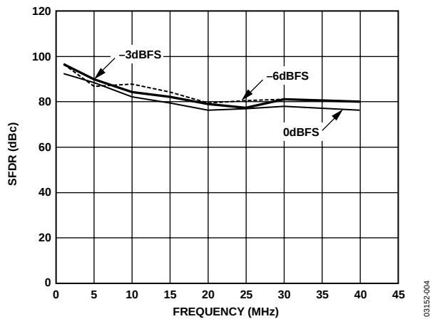
Figure 4. SFDR vs. Frequency, f_{DATA} = 100 MSPS, 4 \times Interpolation
