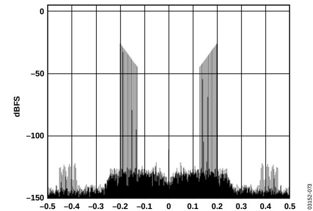
Figure 73. Effects of Hilbert Transform
