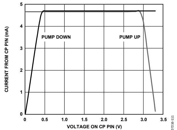
Figure 9. Charge Pump Characteristics at CP_V = 3.3\text{ V}
