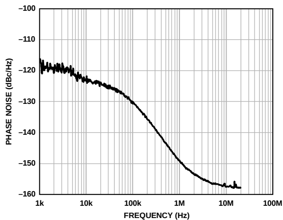
Figure 30. Phase Noise (Absolute) Clock Generation; Internal VCO at 1.966 GHz; PFD = 15.36 MHz; LBW = 40 kHz; LVPECL Output = 122.88 MHz
