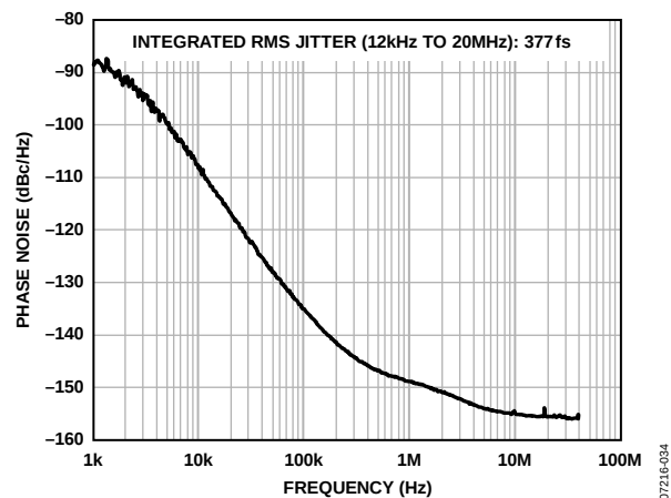
Figure 32. Phase Noise (Absolute) Clock Cleanup; Internal VCO at 1.866 GHz; PFD = 120 kHz; LBW = 1.84 kHz; LVPECL Output = 155.52 MHz
