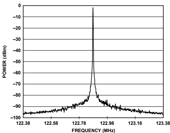
Figure 14. Output Spectrum, LVPECL; 122.88 MHz; PFD = 15.36 MHz; LBW = 127 kHz; I_{CP} = 3.0 mA; f_{VCO} = 1966.08 MHz
