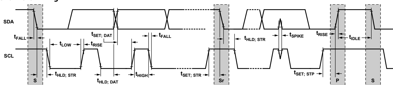
Figure 61. I 2 C Serial Port Timing
