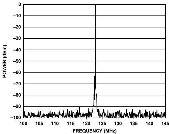
Figure 13. PFD/CP Spurs; 122.88 MHz; PFD = 15.36 MHz; LBW = 127 kHz; I_{CP} = 3.0 mA; f_{VCO} = 1966.08 MHz
