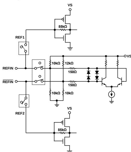
Figure 43. REF1N Equivalent Circuit for Non-XTAL Mode
