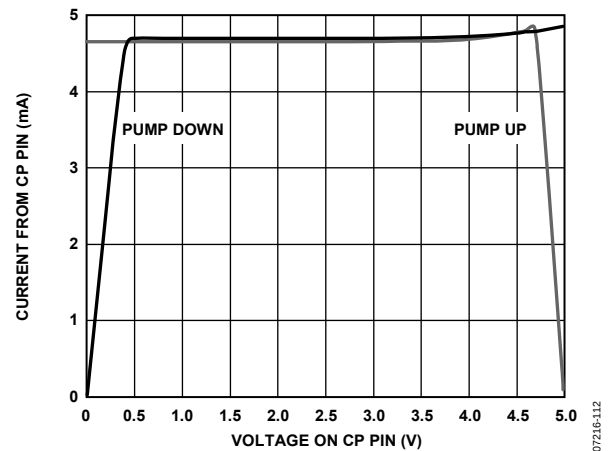
Figure 10. Charge Pump Characteristics at CP_V = 5.0\text{ V}
