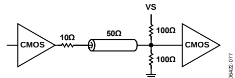
Figure 76. CMOS Output with Far-End Termination
