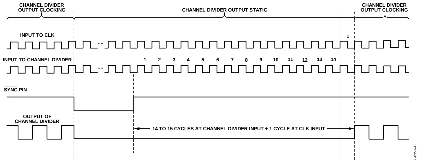
Figure 58. SYNC Timing When VCO Divider Is Not Used—CLK Input Only
