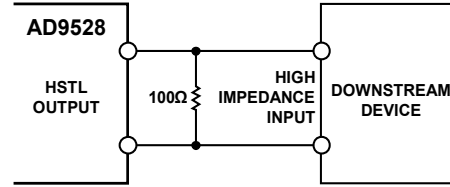
Figure 23. DC-Coupled HSTL Output Driver
