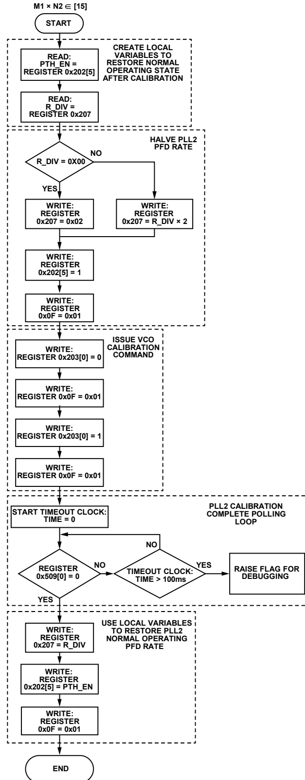
Figure 54. Subprocess, Issue VCO Calibration ( M1 \times N2 = 15 )
