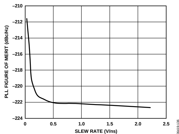
Figure 14. PLL Figure of Merit (FOM) vs. Slew Rate at \text{REFIN}/\text{REFIN}
