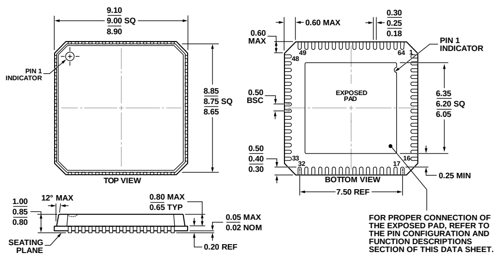
COMPLIANT TO JEDEC STANDARDS MO-220-VMMD-4 Figure 77. 64-Lead Lead Frame Chip Scale Package [LFCSP_VQ] 9 mm x 9 mm Body, Very Thin Quad CP-64-4 Dimensions shown in millimeters
