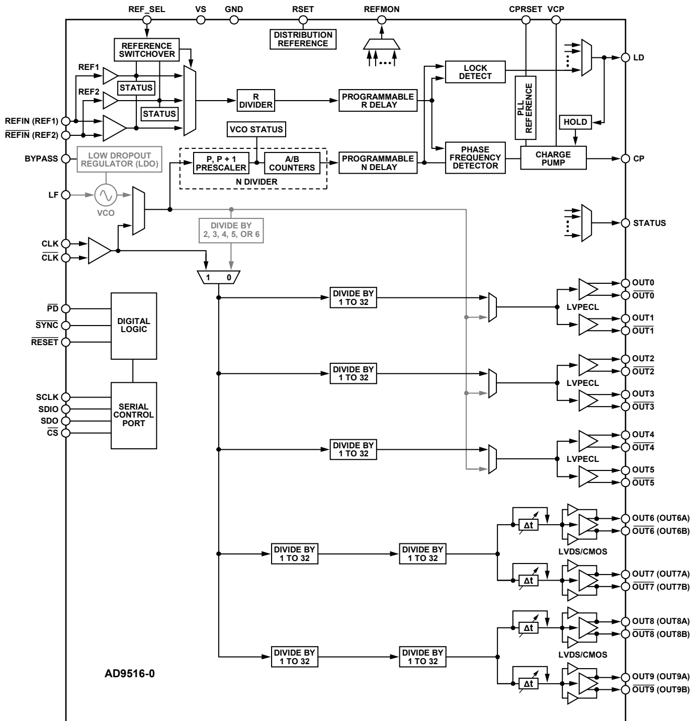
Figure 45. Clock Distribution or External VCO &lt; 1600 MHz
