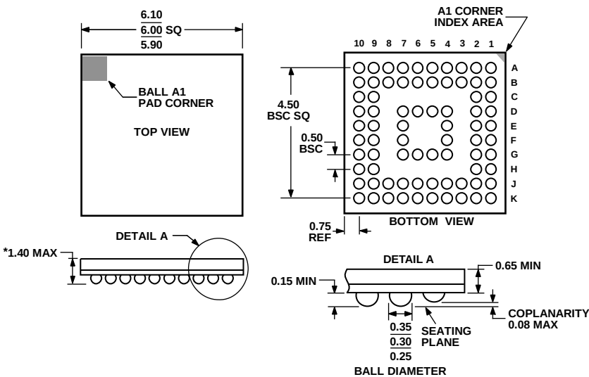
*COMPLIANT TO JEDEC STANDARDS MO-225 WITH THE EXCEPTION TO PACKAGE HEIGHT. Figure 9. 76-Pin Chip Scale Package Pin Grid Array [CSP_BGA] 6 mm × 6 mm × 1.2 mm (BC-76-2) Dimensions shown in millimeters
