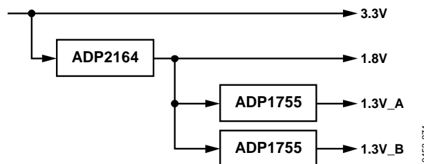
Figure 74. Low Noise Power Solution for the AD9361
