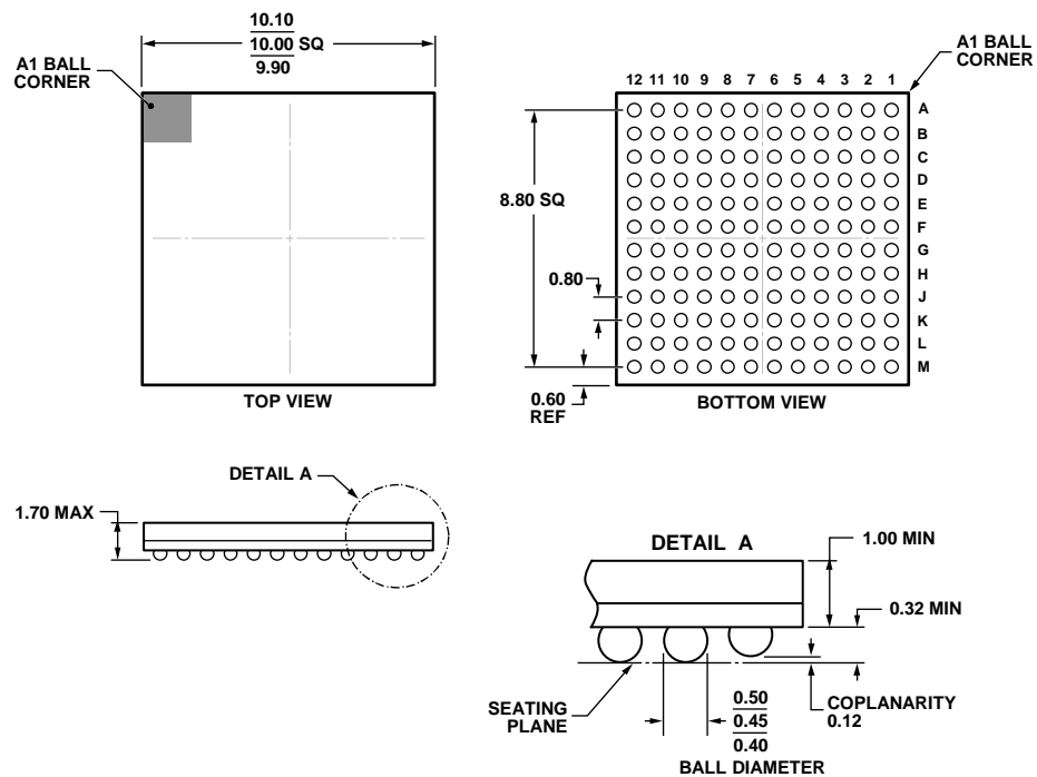
COMPLIANT TO JEDEC STANDARDS MO-275-EEAB-1. Figure 76. 144-Ball Chip Scale Package Ball Grid Array [CSP_BGA] (BC-144-7) Dimensions shown in millimeters
