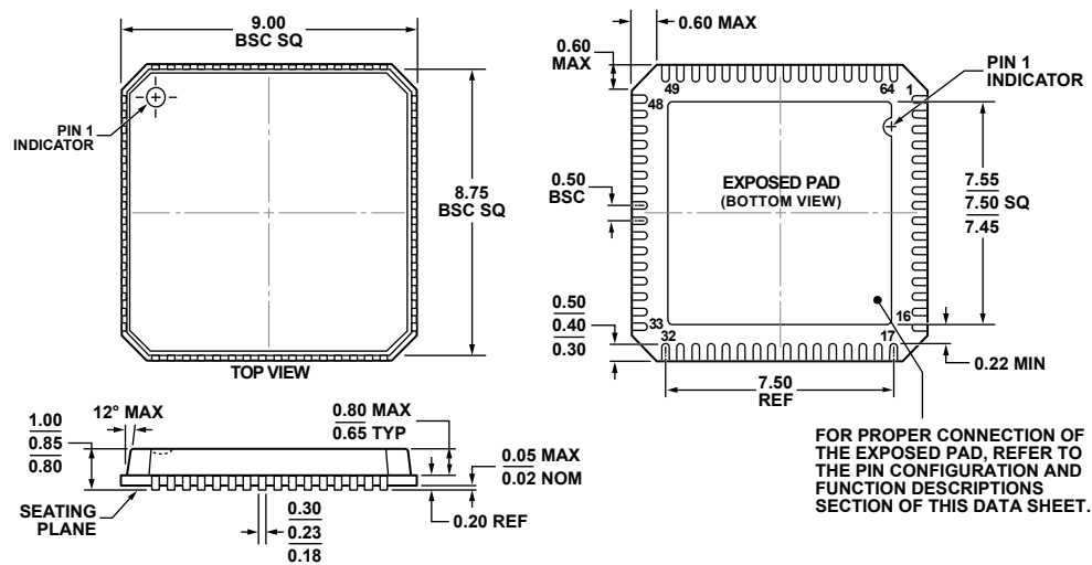
COMPLIANT TO JEDEC STANDARDS MO-220-VMMD-4 Figure 73. 64-Lead Lead Frame Chip Scale Package [LFCSP_VQ] 9 mm x 9 mm Body, Very Thin Quad (CP-64-6) Dimensions shown in millimeters
