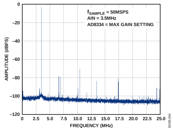
Figure 61. AD9252 FFT Example Results Using 16 MHz, Two-Pole Low-Pass Filter Applied to the AD8334 Outputs (Analog Input Signal = -1.03 dBFS, SNR = 60.2 dBc, SFDR = 66.23 dBc)
