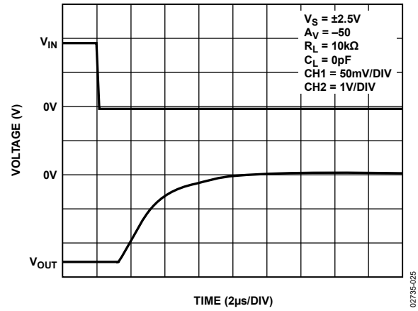
Figure 27. Positive Overtolerance Recovery
