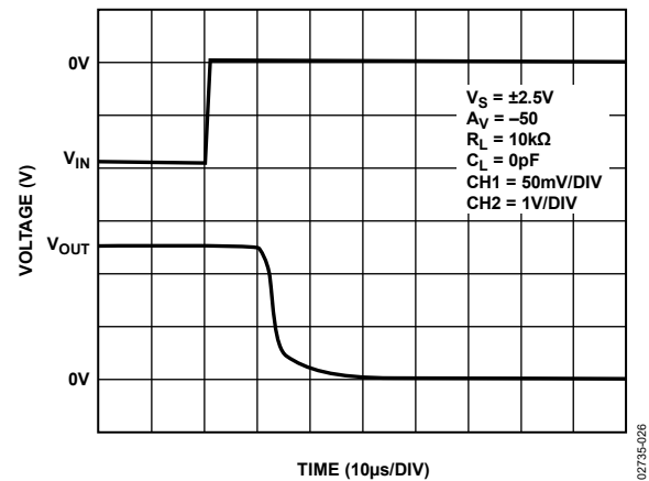
Figure 28. Negative Overtolerance Recovery
