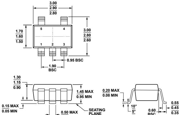
COMPLIANT TO JEDEC STANDARDS MO-178-AA
