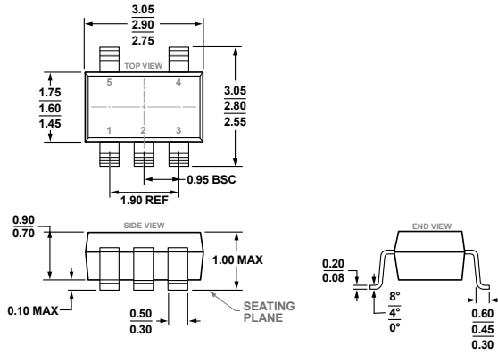
COMPLIANT TO JEDEC STANDARDS MO-193-AB
