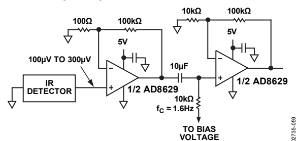
Figure 62. AD8629 Used as Preamplifier for Thermopile
