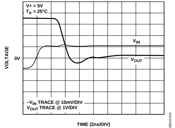
Figure 22. Falling Edge Response
