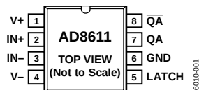
Figure 4. 8-Lead Narrow Body SOIC Pin Configuration
