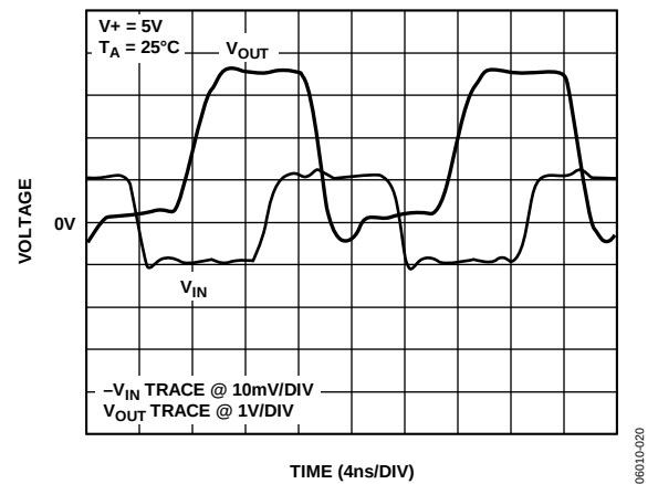
Figure 23. Response to a 50\text{ MHz} , 100\text{ mV} Input Sine Wave
