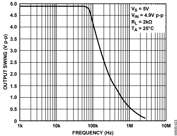
Figure 24. Closed-Loop Output Voltage Swing vs. Frequency
