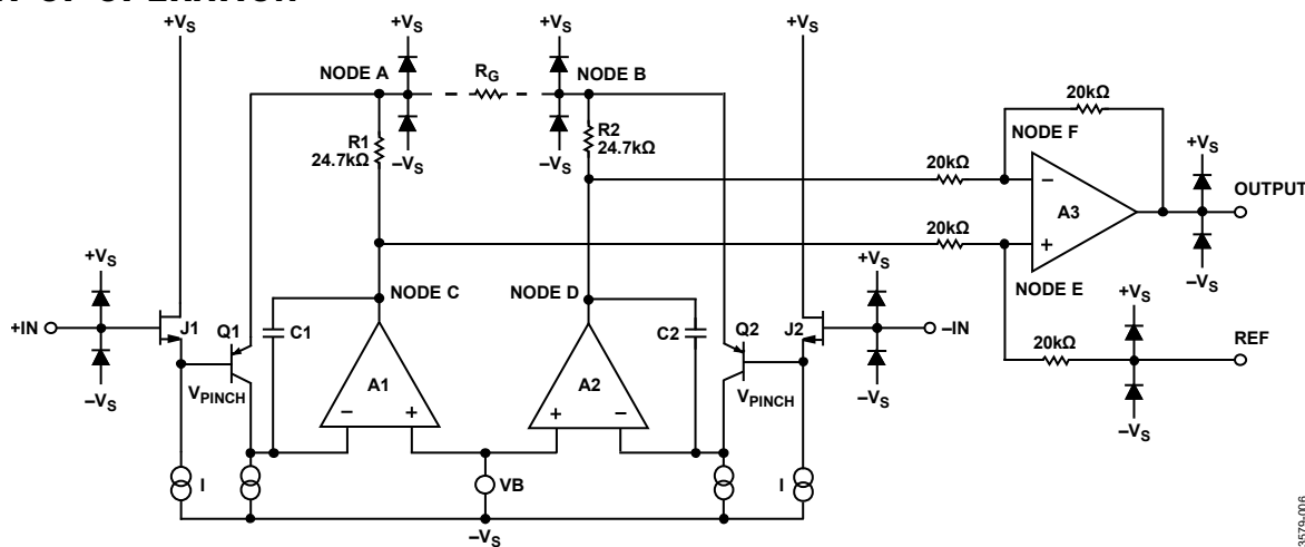
Figure 55. Simplified Schematic
