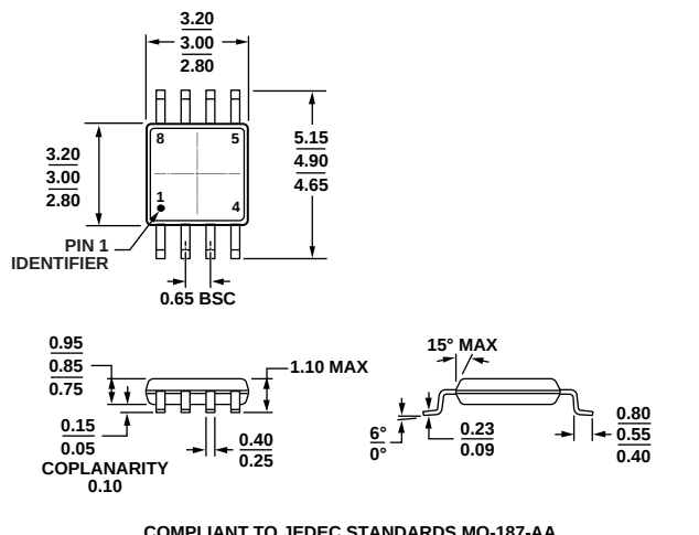
Figure 68. 8-Lead Mini Small Outline Package [MSOP] (RM-8)
