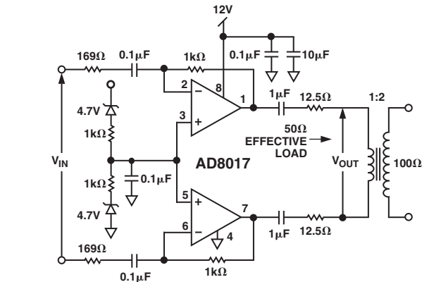
Figure 7. Single 12 V Supply ADSL Remote Terminal Transmitter
