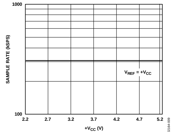
Figure 9. Maximum Sample Rate vs. +V_{\text{CC}}
