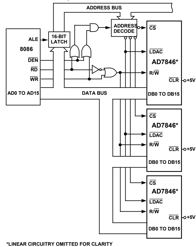
Figure 27. AD7846-to-8086 Interface: Multiple DAC System
