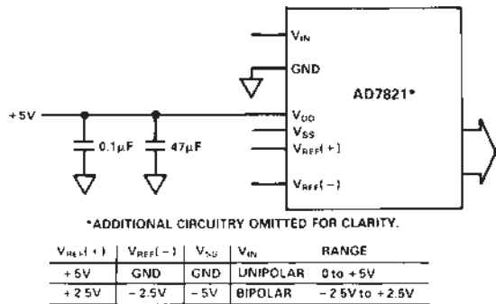
Figure 18. Unipolar/Bipolar Operation
