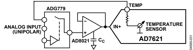
Figure 29. Use of the Temperature Sensor
