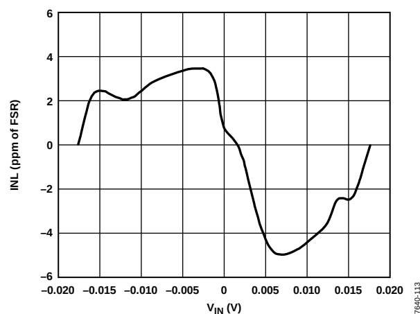
Figure 13. INL (Gain = 128)
