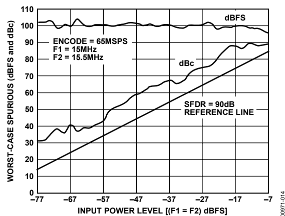
Figure 14. Two-Tone SFDR
