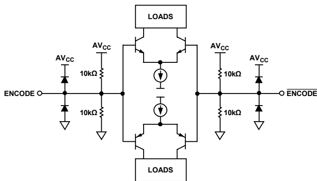
Figure 22. ENCODE/ENCODE-bar Inputs
