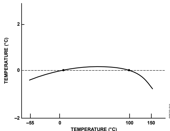
Figure 14. Typical 2-Trim Accuracy
