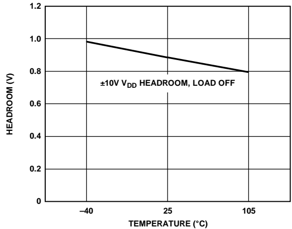
Figure 15. V_{DD} Headroom, \pm 10V Range, Output Set to 10V, Load Off
