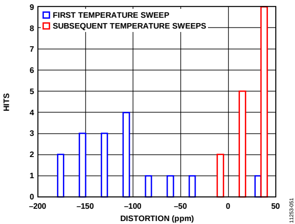
Figure 48. Thermal Hysteresis
