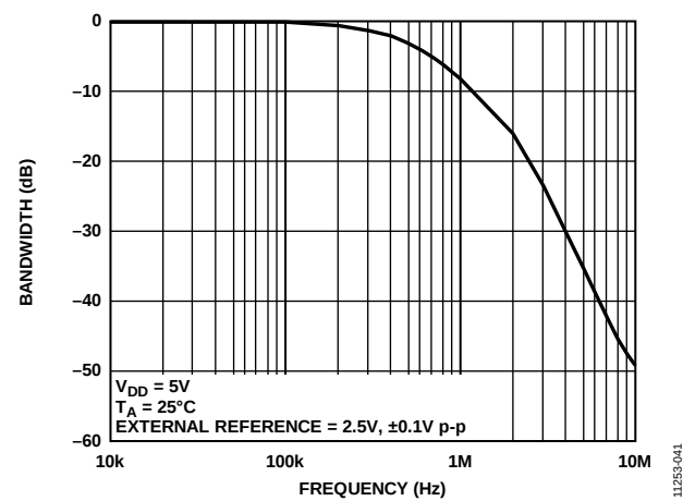
Figure 39. Multiplying Bandwidth, External Reference = 2.5 V, \pm 0.1 V p-p, 10 kHz to 10 MHz
