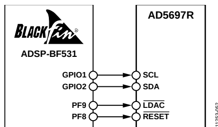
Figure 49. ADSP-BF531 Interface to the AD5697R
