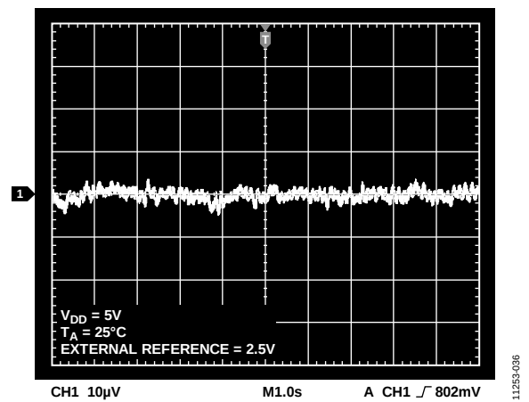
Figure 34. 0.1 Hz to 10 Hz Output Noise Plot, External Reference
