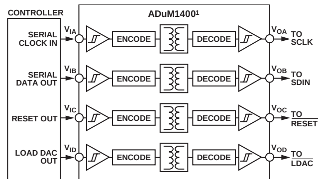
Figure 51. Isolated Interface
