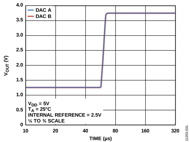
Figure 29. Settling Time
