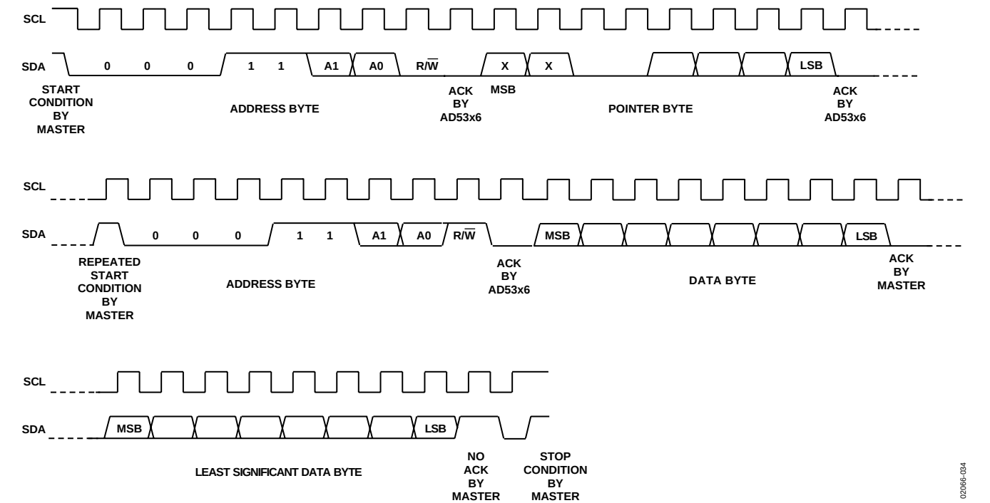
Figure 34. Readback Sequence
