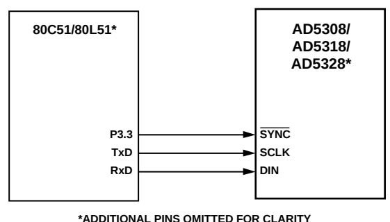
Figure 38. 80C51/80L51-to-AD5308/AD5318/AD5328 Interface
