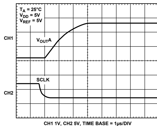
Figure 20. Half-Scale Settling ( \frac{1}{4} to \frac{3}{4} Scale Code Change)
