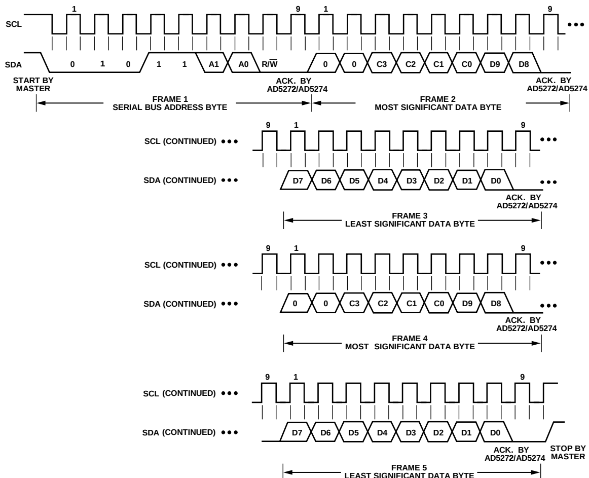
Figure 44. Multiple Write
