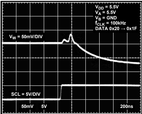
Figure 21. Midscale Glitch Energy
